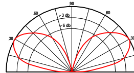
1/2 Wave Dipole Vertical Pattern
