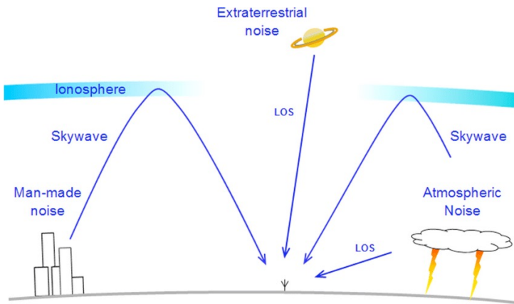
Background Noise
