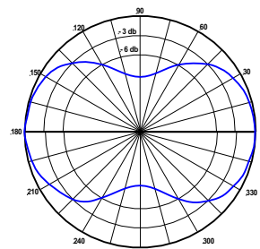
1/2 Wave Dipole Horizontal Pattern
