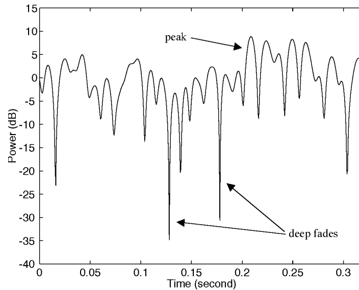
Signal Fading
