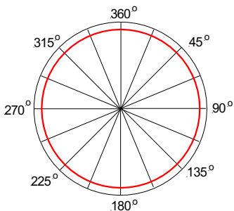
Horizontal Radiation Pattern Vertical Antenna
